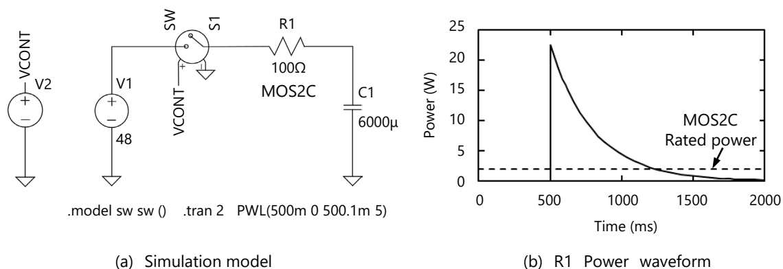
Fig.1 Simulation of pre-charge circuit
