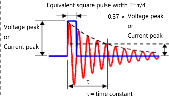
Fig.6 Methods of conversion to equivalent square waves
