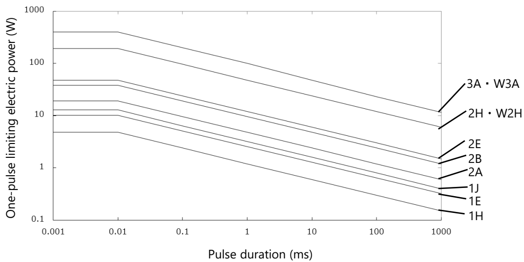
Fig.4 One-pulse limiting electric power of RK73B
