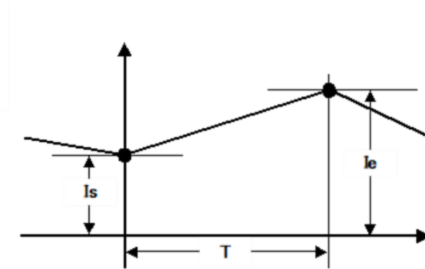
Fig.8 Calculation of energy by interval integration (with current)
