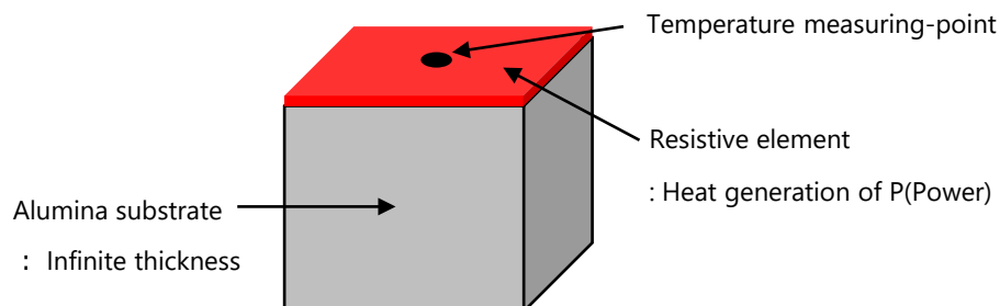
Fig.11 Simplified model for confirmation of temperature rise
