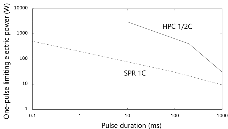
Fig.2 One-pulse limiting electric power diagram of HPC 1/2C and SPR 1C
