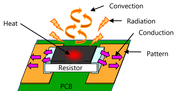
Fig.10 Image of heat generation and heat release of resistor
