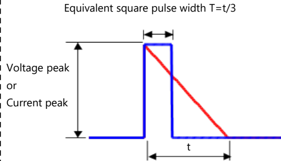
( ii ) Triangular waveform
