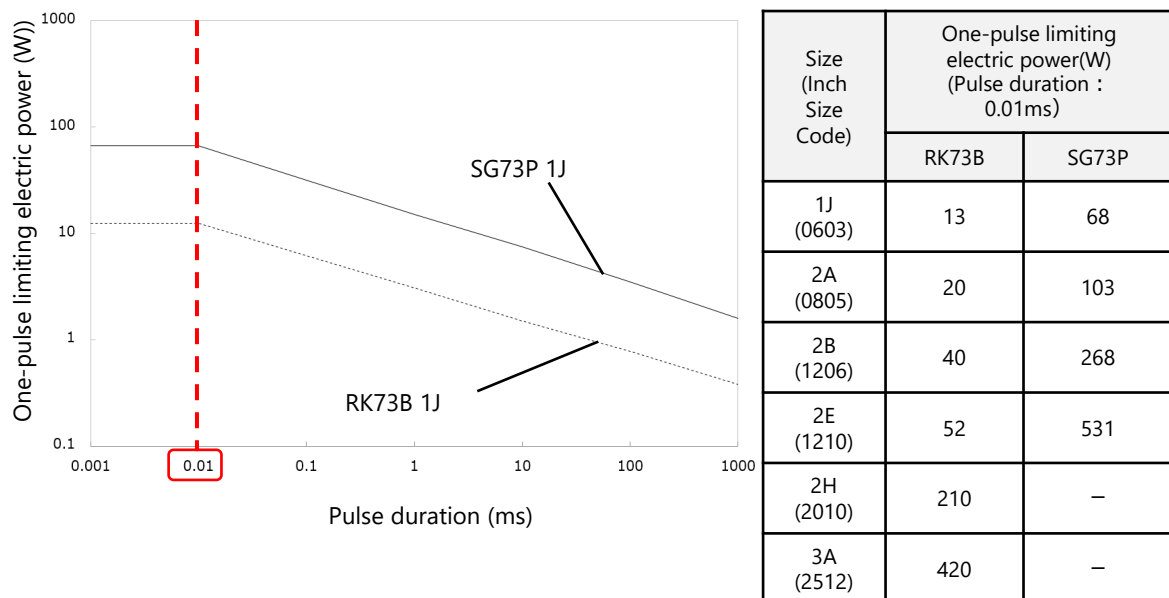
Fig.14 One-pulse limiting electric powers by type and size of resistors
