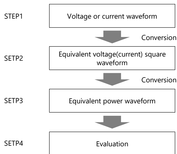
Fig.5 Evaluation procedure of pulse power capability
