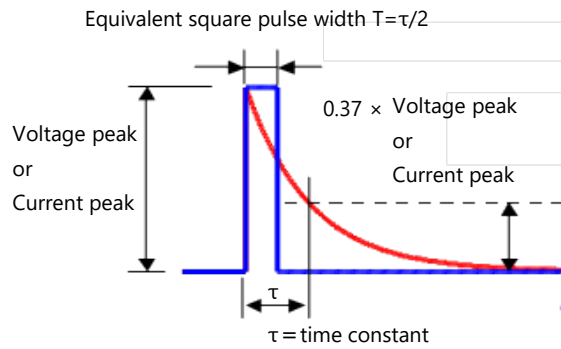
( i ) CR discharge waveform
