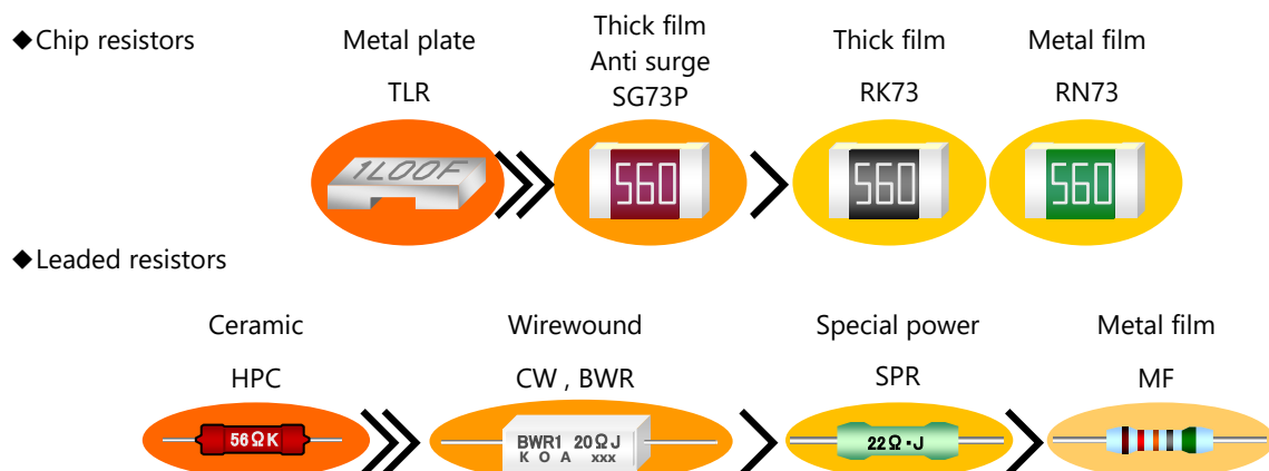
Fig.3 Types of resistors and pulse power capabilities
