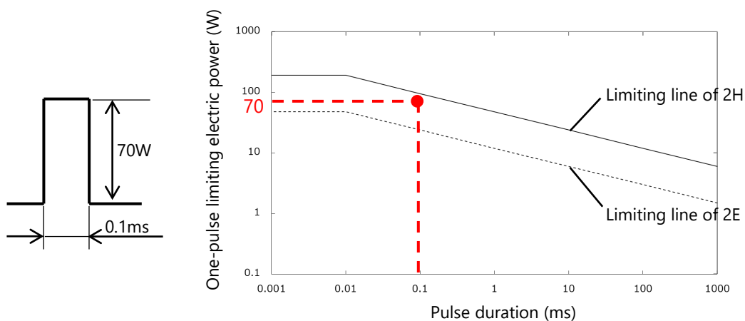
Fig.9 Example of evaluation using one-pulse limiting electric power of thick film chip resistor (RK73B)
