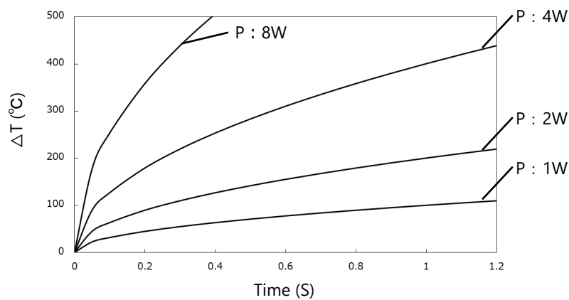
Fig.12 Temperature rise in resistor body resulting from electric power
