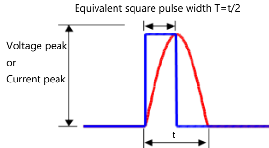
( iii ) Half-wave sinusoidal waveform
