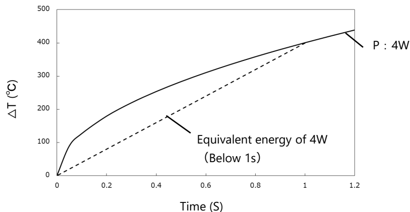
Fig.13 Comparison between calculation using equation (2) and equivalent energy conversion
